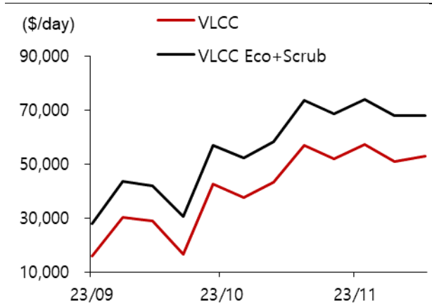
[조선] 탱커(Tanker)_VLCC 운임
