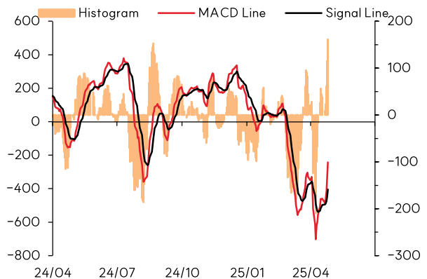
나스닥 MACD
