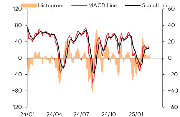
나스닥 MACD
